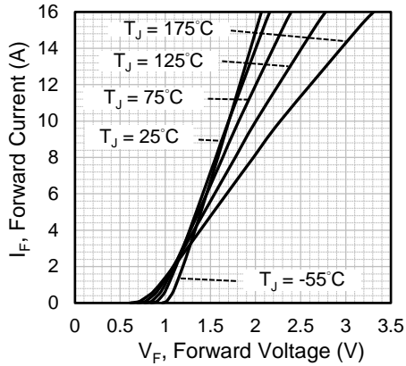
Fig.1 Forward Characteristics
