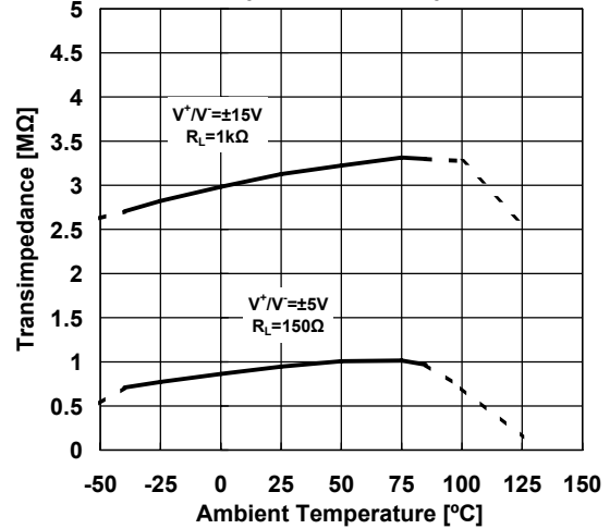
Transimpedance vs. Temperature
