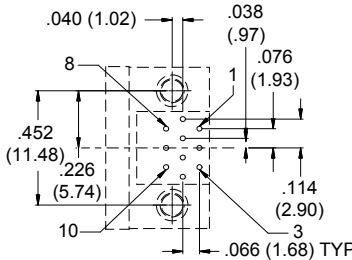
PCB FOOTPRINT
