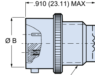
Accessory Thread 803-004-01
