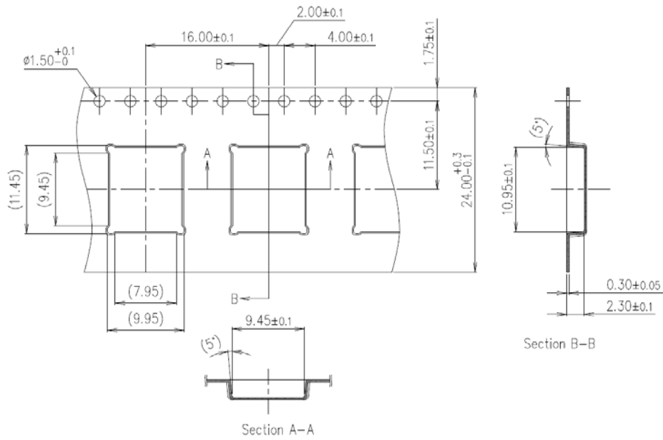
Figure 36. Tape Dimension
