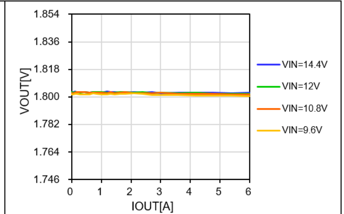
Figure 12. V_{OUT} vs. Load Current and Line Voltage
