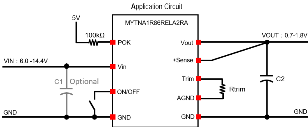
Figure 33. Application Schematic
