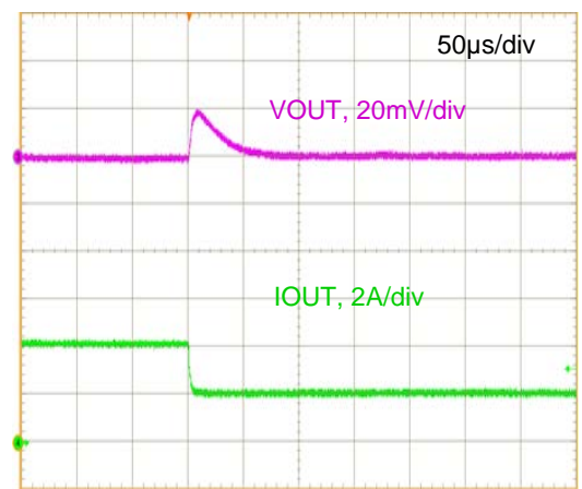
Figure 22. Step Load Transient Response
