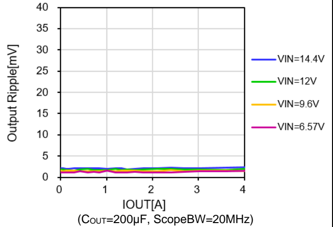
Figure 20. Output Ripple and Noise
