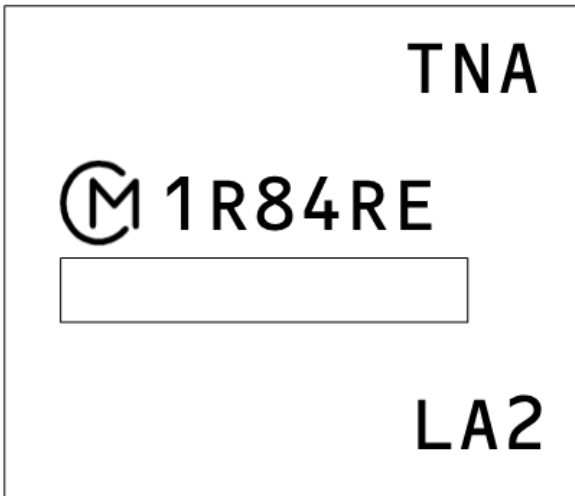
Figure 32. Top Marking Specification
