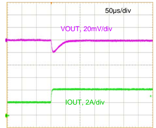
Figure 21. Step Load Transient Response
