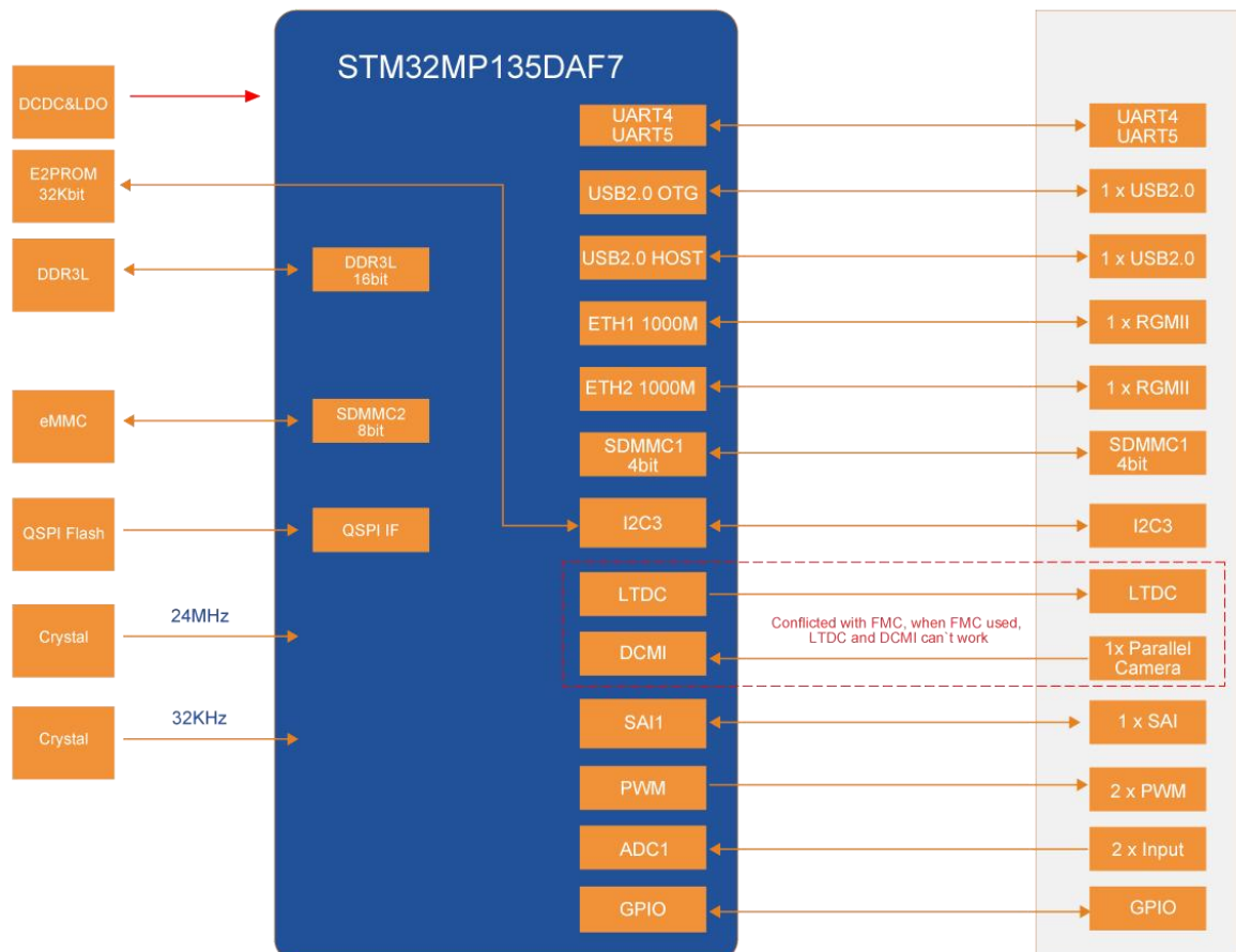
MYC-YF13X CPU Module Function Block Diagram
