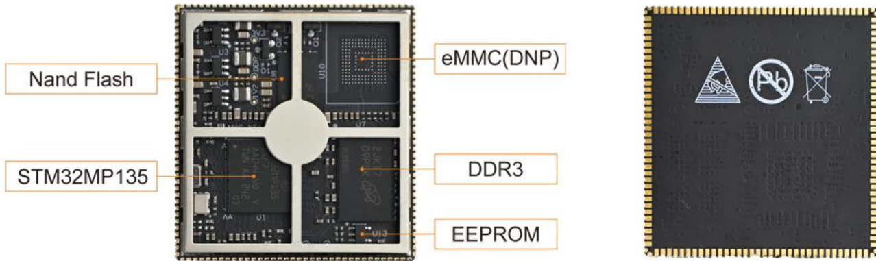
MYC-YF13X CPU Module Top-view and Bottom-view (delivered with shielding cover installed by default)
