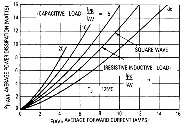
Figure 15. Power Dissipation
