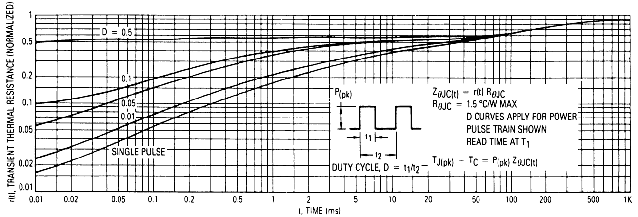
Figure 16. Thermal Response
