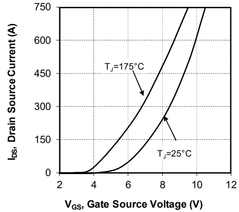
Figure 1-5. Transfer Characteristics
