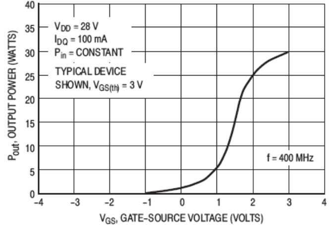
Figure 17. Output Power versus Gate Voltage
