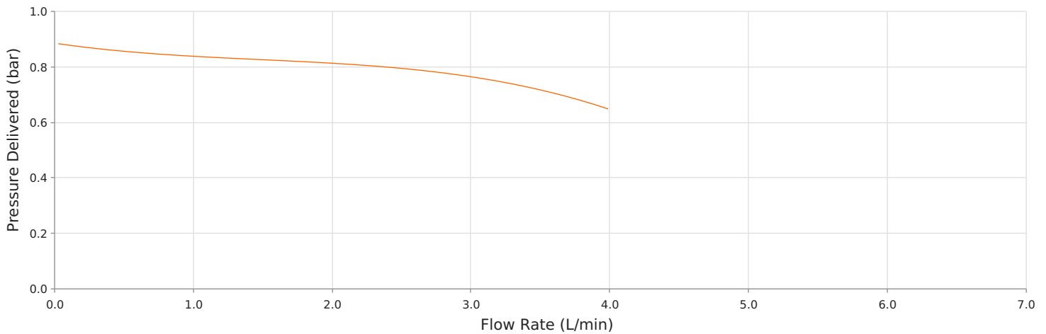
MRC150-DH2-HT-DV - Pump Capacity
