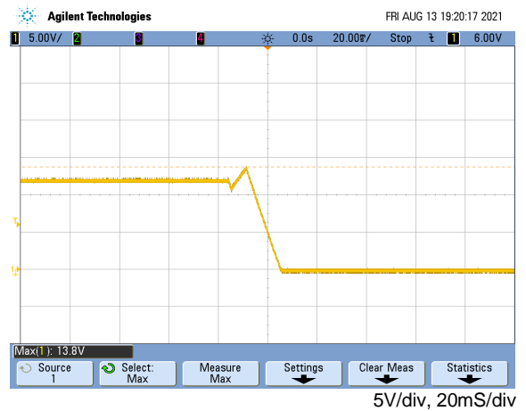
OVP 60% of rated load
