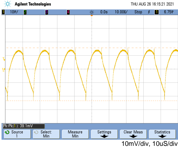
Switching frequency ripple rated load
