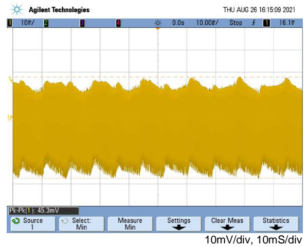
Line frequency ripple rated load
