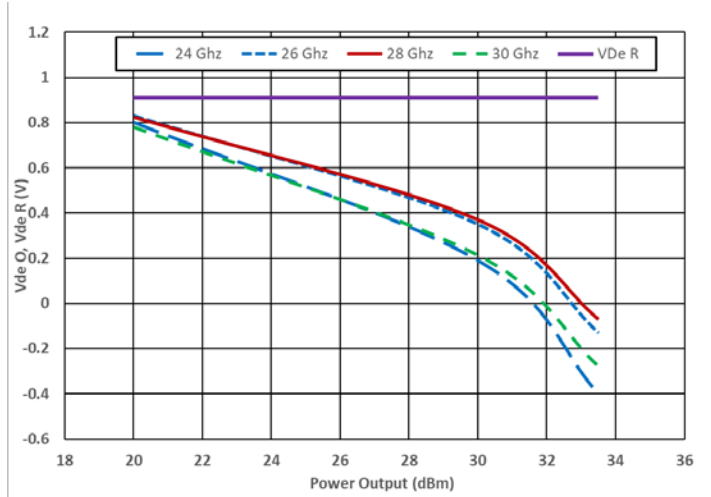
Detector Output vs. Output Power
