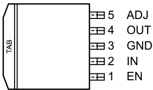
MIC69301/2 5-Lead S-PAK (R) Adjustable Voltage
