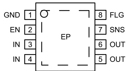
MIC69301/3 8-Lead ePad SOIC (ME) Fixed Voltage with Flag
