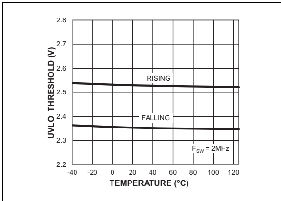
FIGURE 2-3: UVLO Threshold vs. Temperature.
