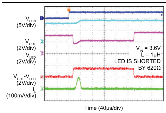
FIGURE 2-20: LED Short-Circuit Protection (LED is Shorted by 620\Omega ).
