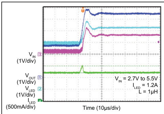
FIGURE 2-27: Line Transient ( V_{IN} Changes from 2.7V to 5.5V).
