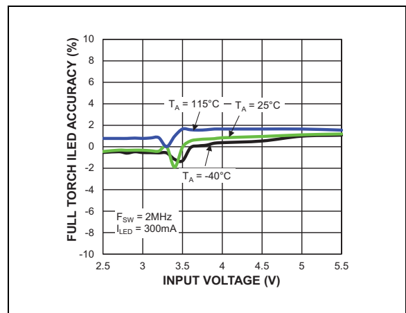
FIGURE 2-11: Full Torch ILED Accuracy vs. Input Voltage.
