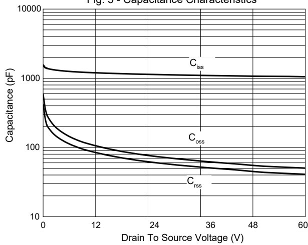
Fig. 5 - Capacitance Characteristics
