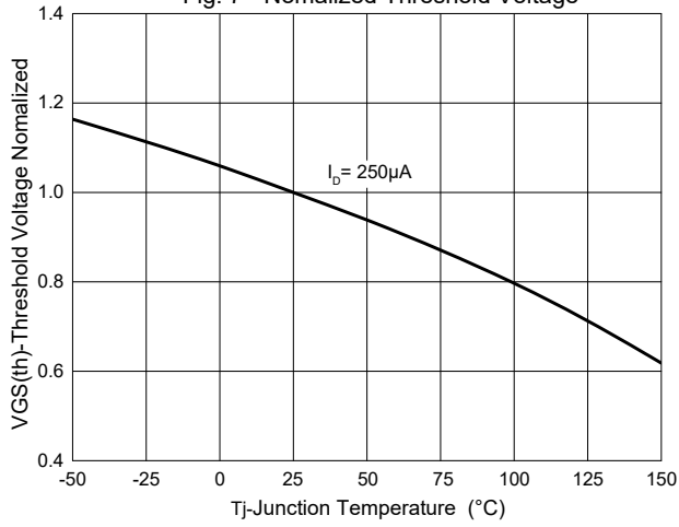
Fig. 7 - Normalized Threshold Voltage
