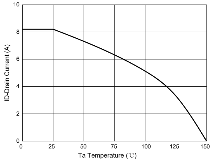
Fig. 10 - Drain Current
