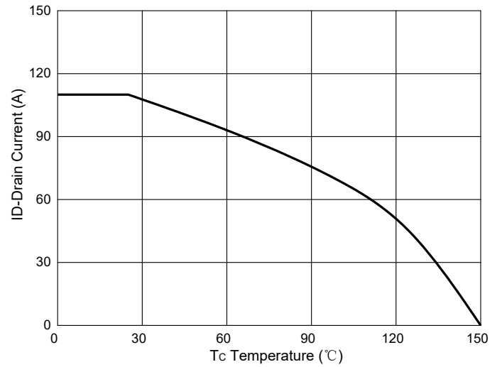
Fig. 10 - Drain Current
