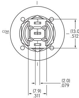
Single Pole
