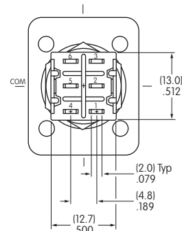
Double Pole
