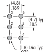
Double Pole
