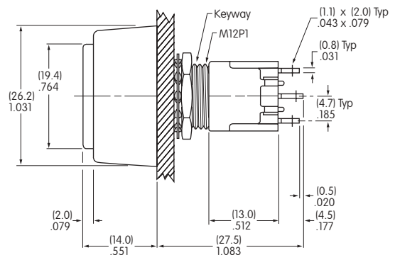
Double Pole
