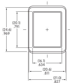
Single Pole
