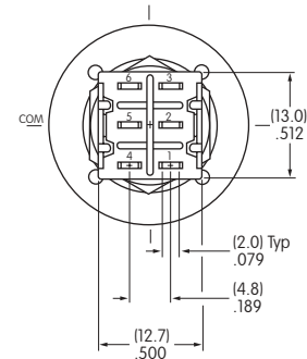
Double Pole
