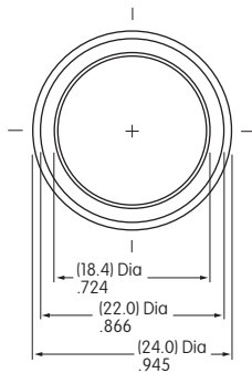
Single Pole
