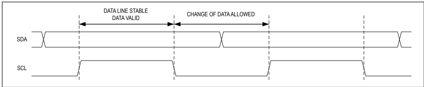
Figure 11. I 2 C Bit Transfer
