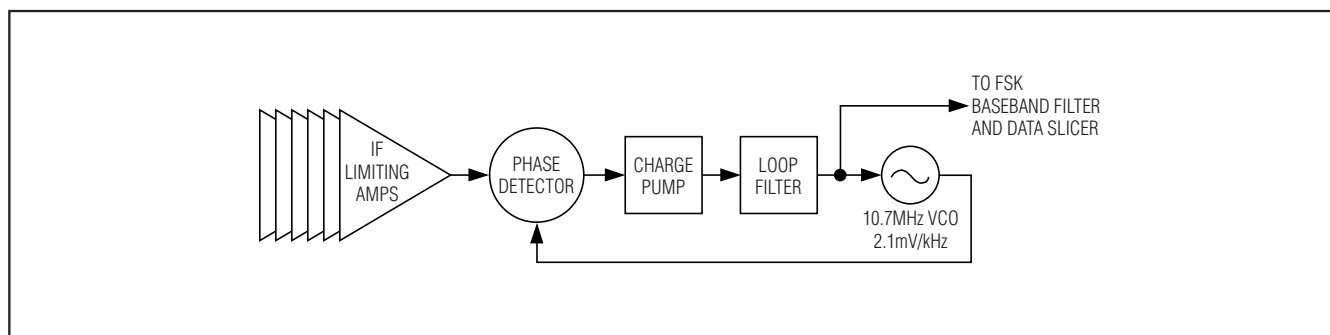
Figure 1. FSK Demodulator PLL Block Diagram
