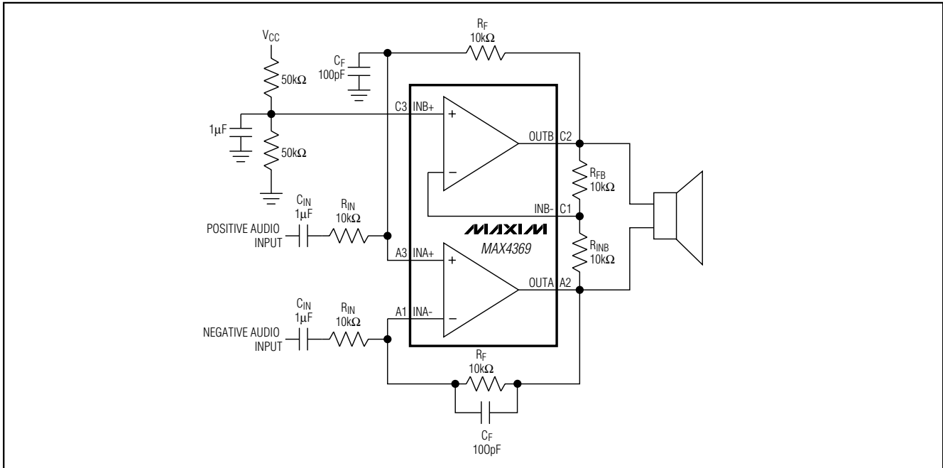
Figure 3. Differential Input/Differential Output Audio Amplifier
