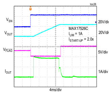
POWER-UP RESPONSE WITH 1000µF CAPACITOR AT NO LOAD
