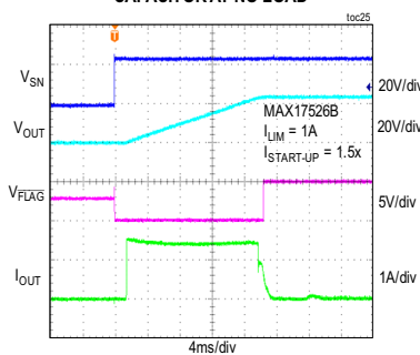
POWER-UP RESPONSE WITH 1000µF CAPACITOR AT NO LOAD
