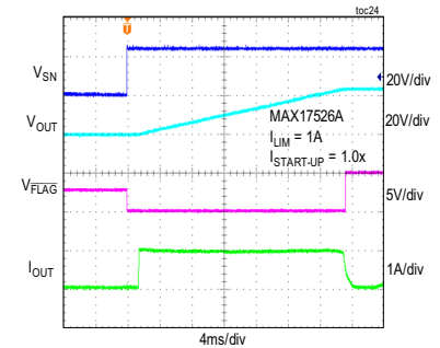
POWER-UP RESPONSE WITH 1000µF CAPACITOR AT NO LOAD
