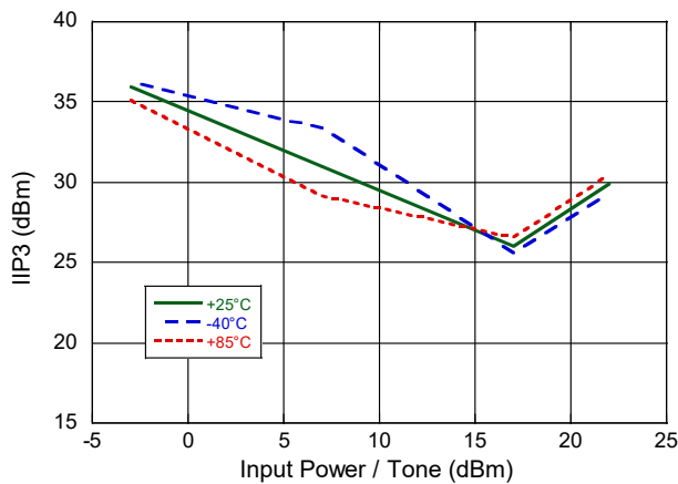
Input IP3 over Temperature @ 8 GHz
