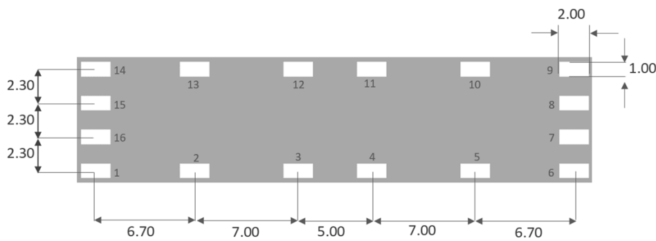
Pads 1-16 = 2.0 x 1.0 (mm)
