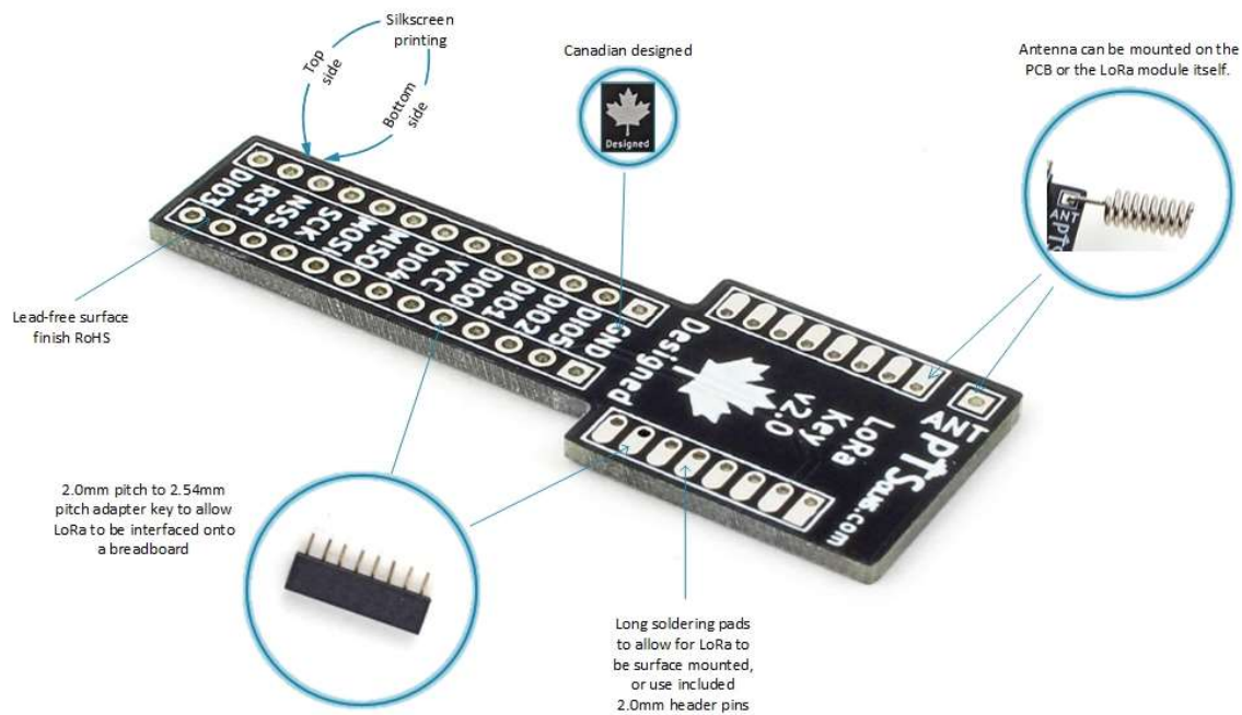
Figure 2: Features of the LoRa Key.
