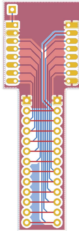
Figure 4: Electrical connections of the LoRa Key.
