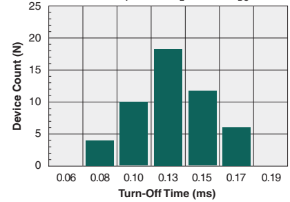
Typical Turn-Off Time (N=50, I_F=5\text{mA} , I_L=120\text{mA}_{DC} )
