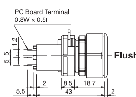
PC Board Terminal
