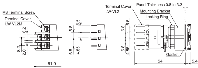
Screw Terminal PC Board Terminal
