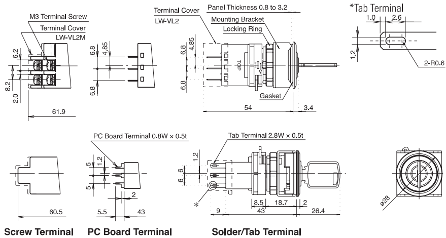
Screw Terminal PC Board Terminal Solder/Tab Terminal
