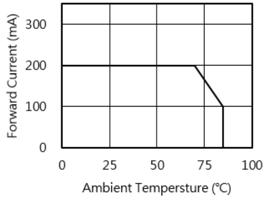
Fig 5. Forward Current Derating Curve
