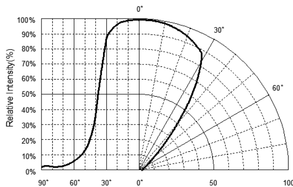
Fig 2. Radiation Characteristics
