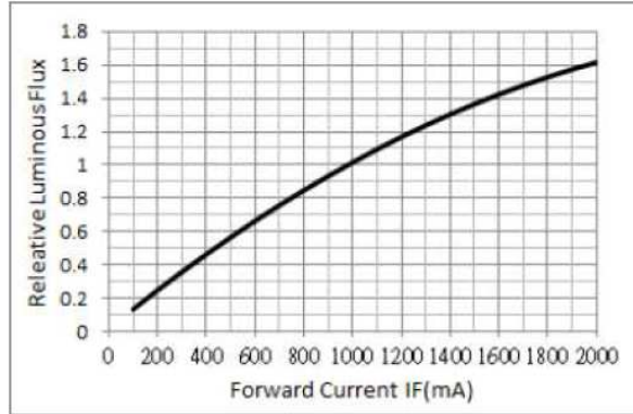
Fig 4. Relative Luminous Flux
