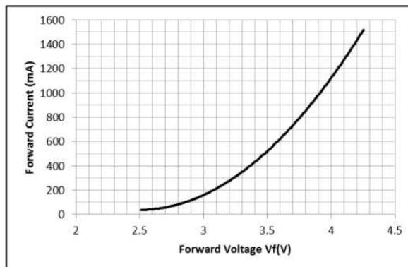
Fig 3. Forward Current
