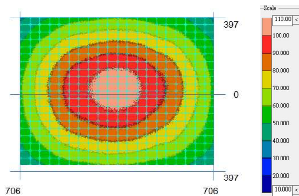
Fig 6. Illumination Profile FOV:78degree(16:9) Unit:mm
