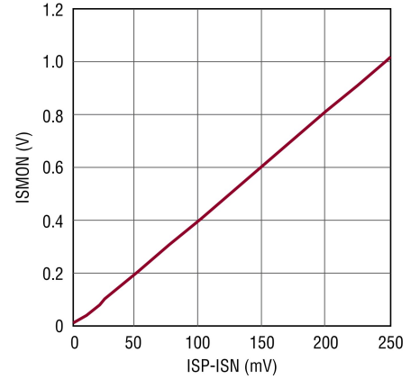
ISMON Voltage vs ISP-ISN Voltage
