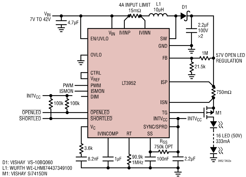
Short LED Protection without R SS : Hiccup Mode
