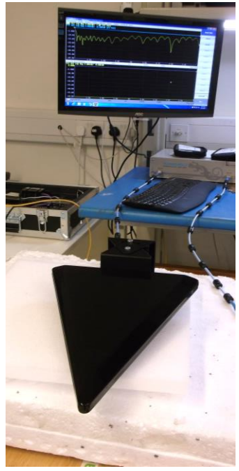
Return Loss and VSWR Measurement
