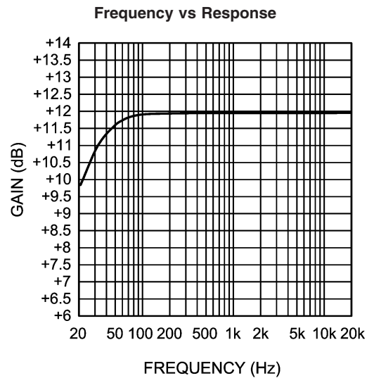
LLS, RLS; R_L = 8\Omega ; Mode 7; Full Gain
