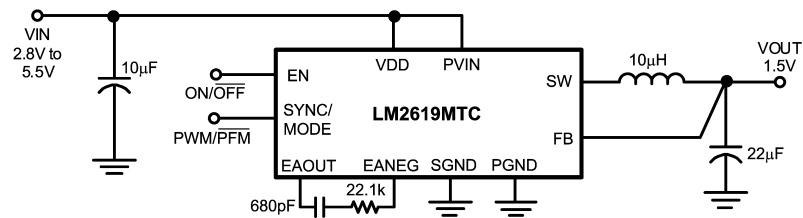
FIGURE 3. Typical Circuit for 1.5V Output Voltage
