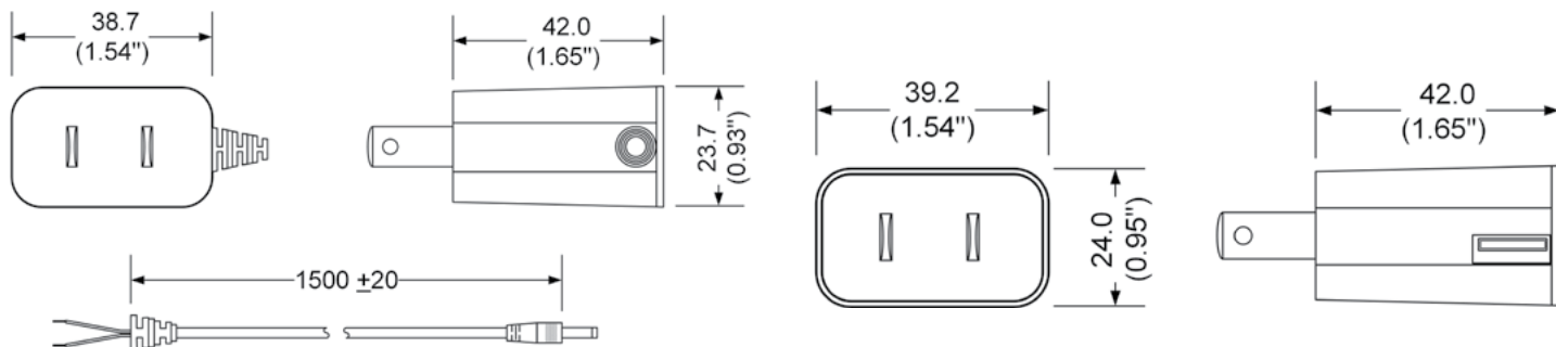
L6R06H-050U Outline Drawing
