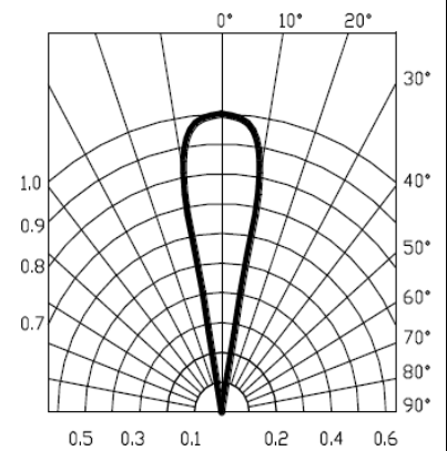
Radiation Diagram
