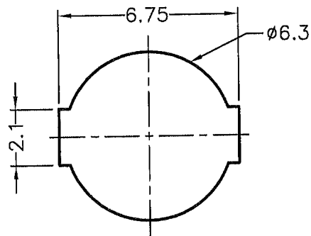
MOUNTING HOLE CHASSIS THICKNESS 0.7mm
