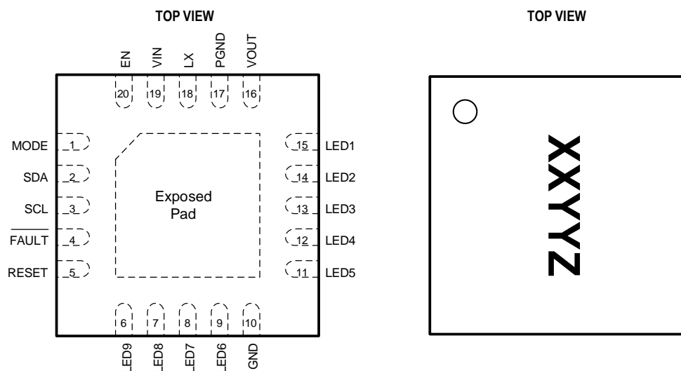
UQFN33-20
