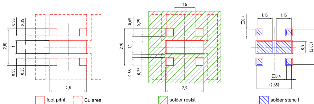
Alternative Solder pad design for pedestal MCPiB
