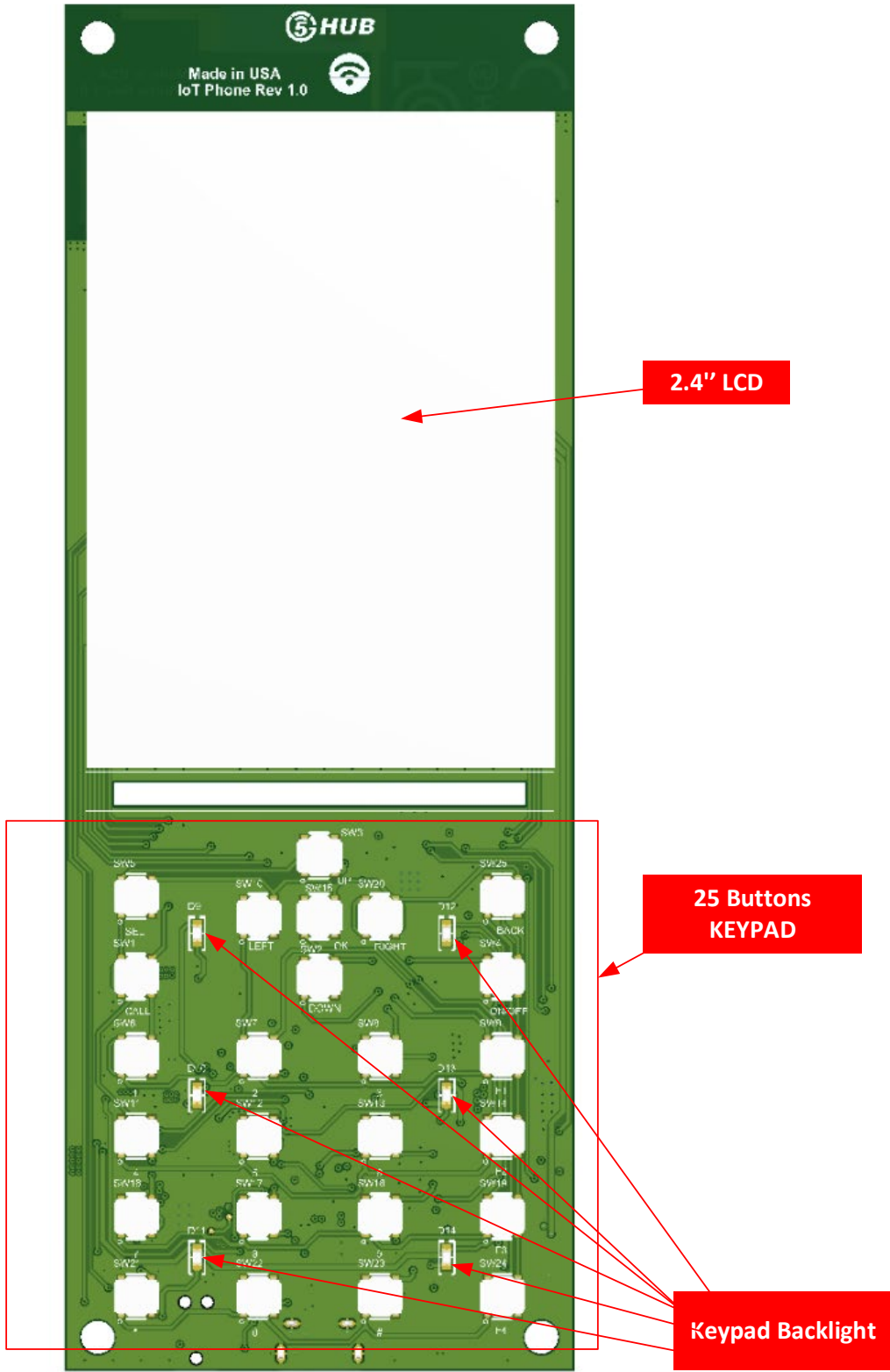
Figure 4. NB-IoT Phone Top Side – Key Components
