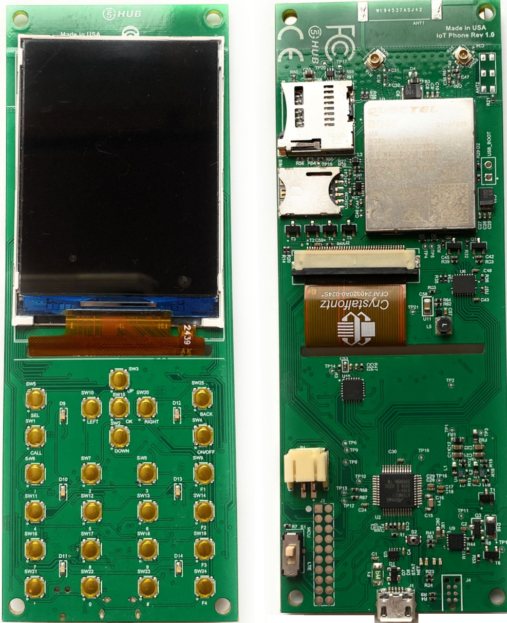
Figure 1. NB-IoT Phone Overview Diagram – Top & Bottom Views
