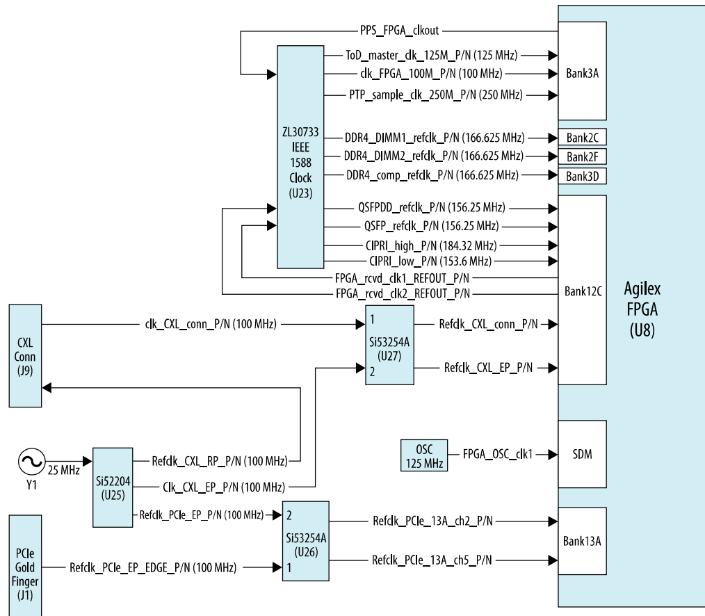
Figure 26. Intel Agilix F-Series FPGA Development Kit Clocks and Default Frequencies
