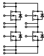
VKM H-Bridge
