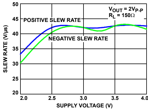
FIGURE 19. SLEW RATE vs SUPPLY VOLTAGE
