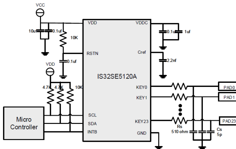
Figure 1 Typical Application Circuit (WQFN-32)
