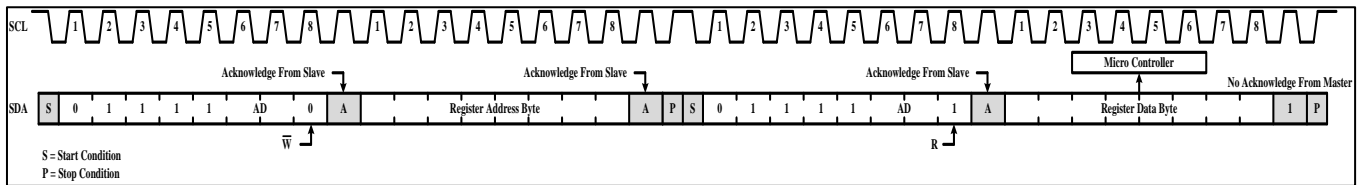
Figure 9: Reading from IS32SE5120A
