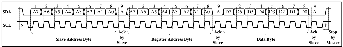
Figure 8: Writing to IS32SE5120A
