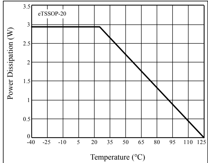
Figure 69 Dissipation Curve
