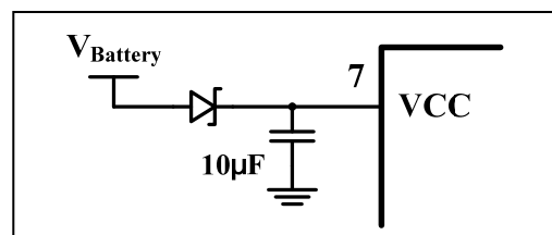
Figure 67 Capacitor For Latch Status
