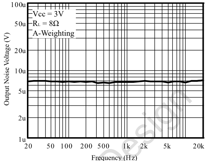
Figure 15 Noise Floor
