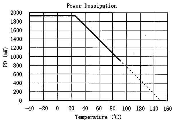
Figure 10. Power Dissipation
