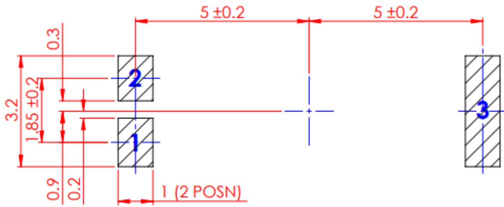
FOOTPRINT PCB
