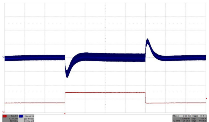
Fig. 25: Output voltage response to load current step change 100% - 50% (7.5A-15A-7.5A) with di/dt = 1A/\mu s at V_{in} = 24V . Top trace (C4): Output voltage (500 mV/div.). Bottom trace (C3): Load current (10 A/div.). C_o = 470 \mu F/70m\Omega . Time: 1ms/div.
