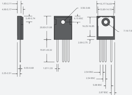
TO-247-4-Lead
