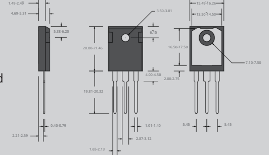
TO-247-3-Lead
