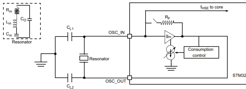
FIGURE 3: EXTERNAL OSCILLATOR CIRCUIT DIAGRAM.
