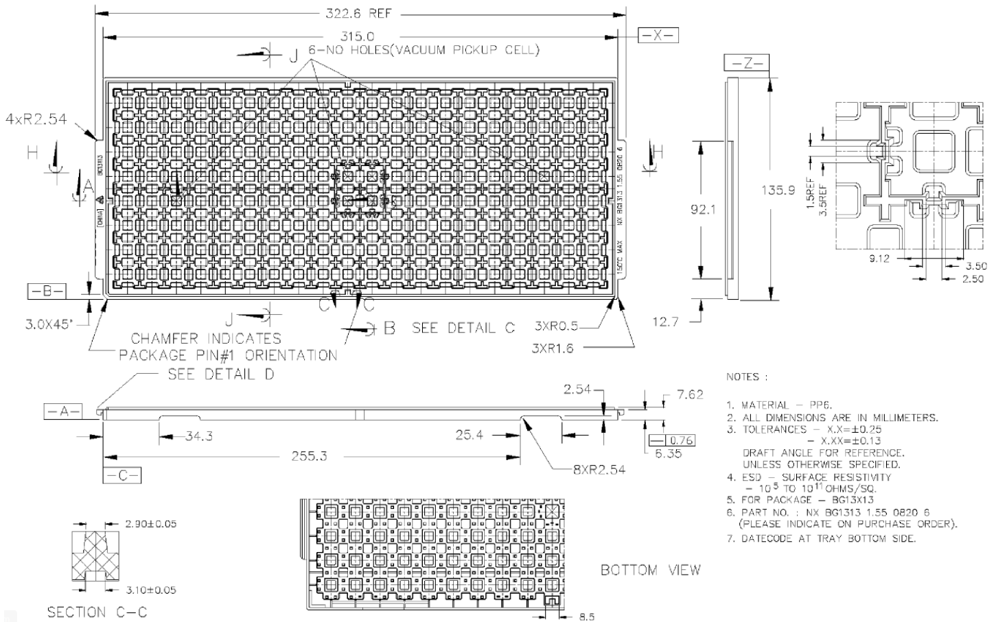
FIGURE 7: TRAY SIZES
