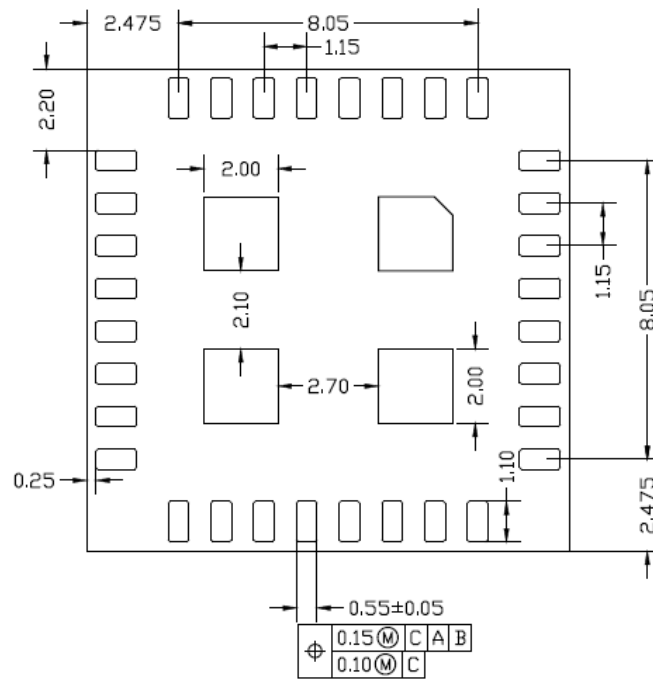
FIGURE 5: PACKAGE OUTLINE
