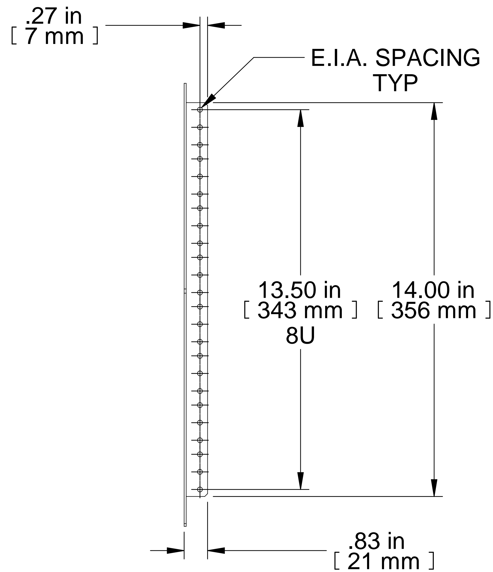
FRONT VIEW
